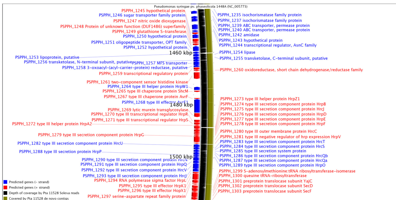
Figure 2 Conservation of the Hrp pathogenicity island between Pph I448A and Pta I1528. Panel A shows an alignment of the Pph I448A Hrp pathogenicity island (lower track) against the homologous region in Pta I1528 (upper track), prepared using GenomeMatcher, which indicates similarity values by colour with dark blue, green, yellow and red representing increasing degrees of similarity [78]. Panel B shows the MAQ [79] alignment of the Pta I1528 Illumina reads (in black) and the BLASTN [80] alignment of the Pta I1528 de novo assembly (in green) against the Hrp region of the Pph I448A genome.
